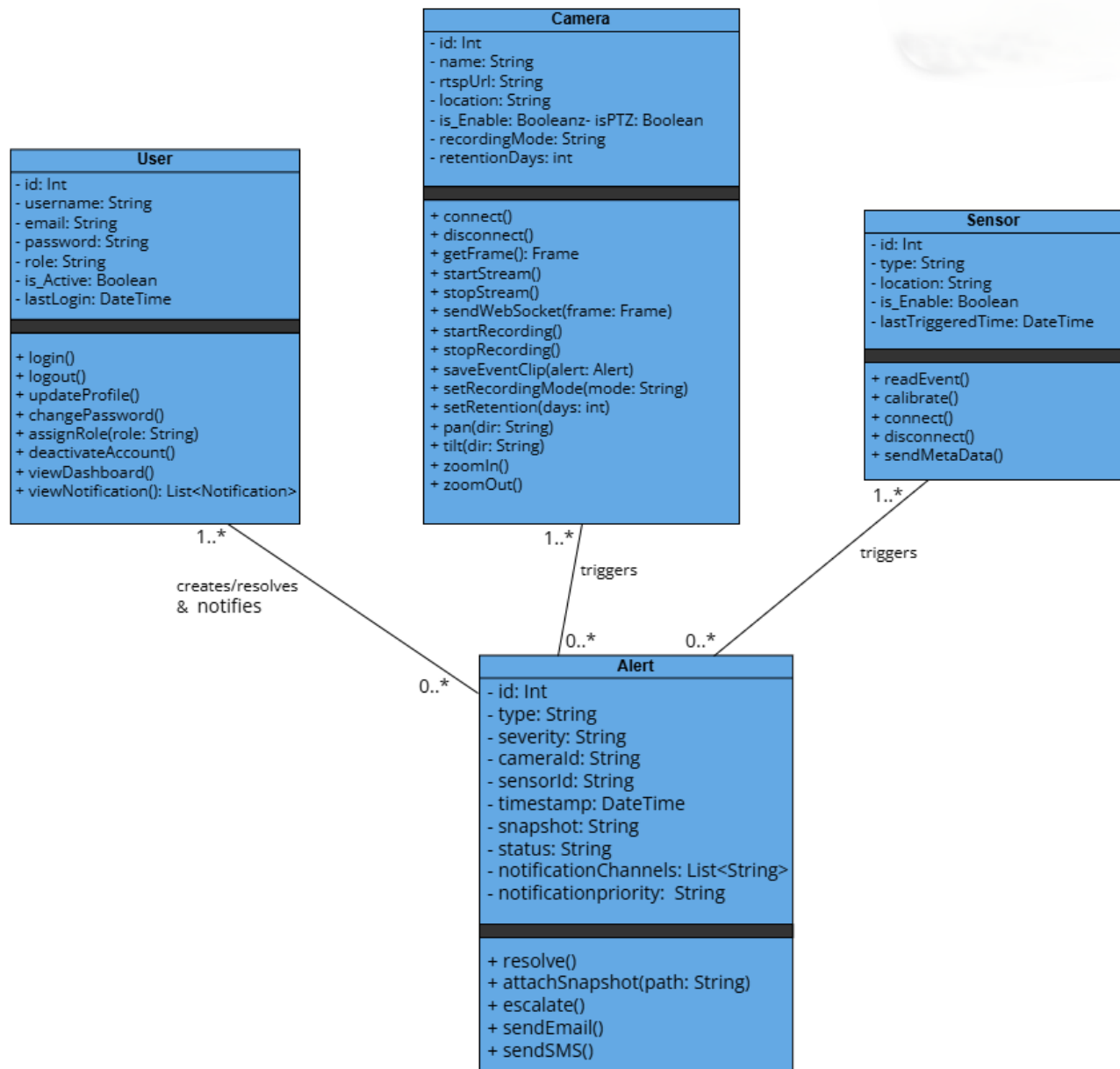
Figure 3.5 : Class Diagram
