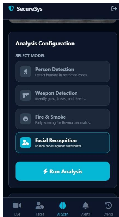
Figure 4.23 : AI Scan UI
