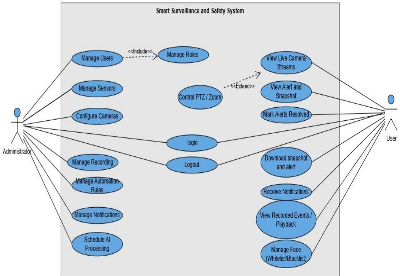
Figure 3.1: Use Case Diagram
