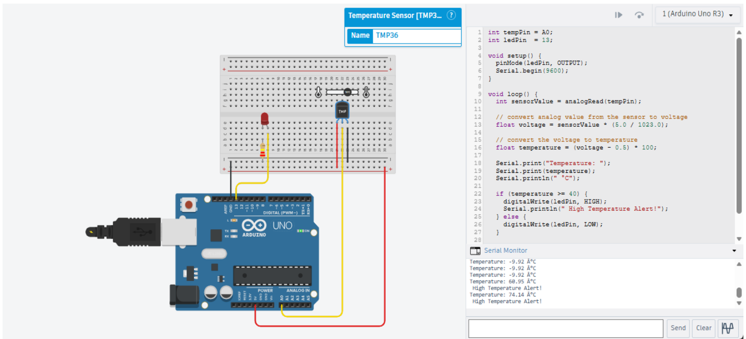
Figure 4.3 : Temperature Sensor
