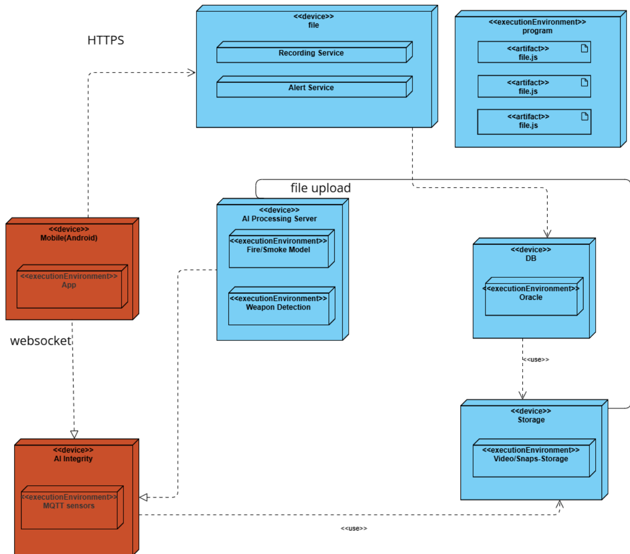
Figure 3.11 : Deployment Diagram
