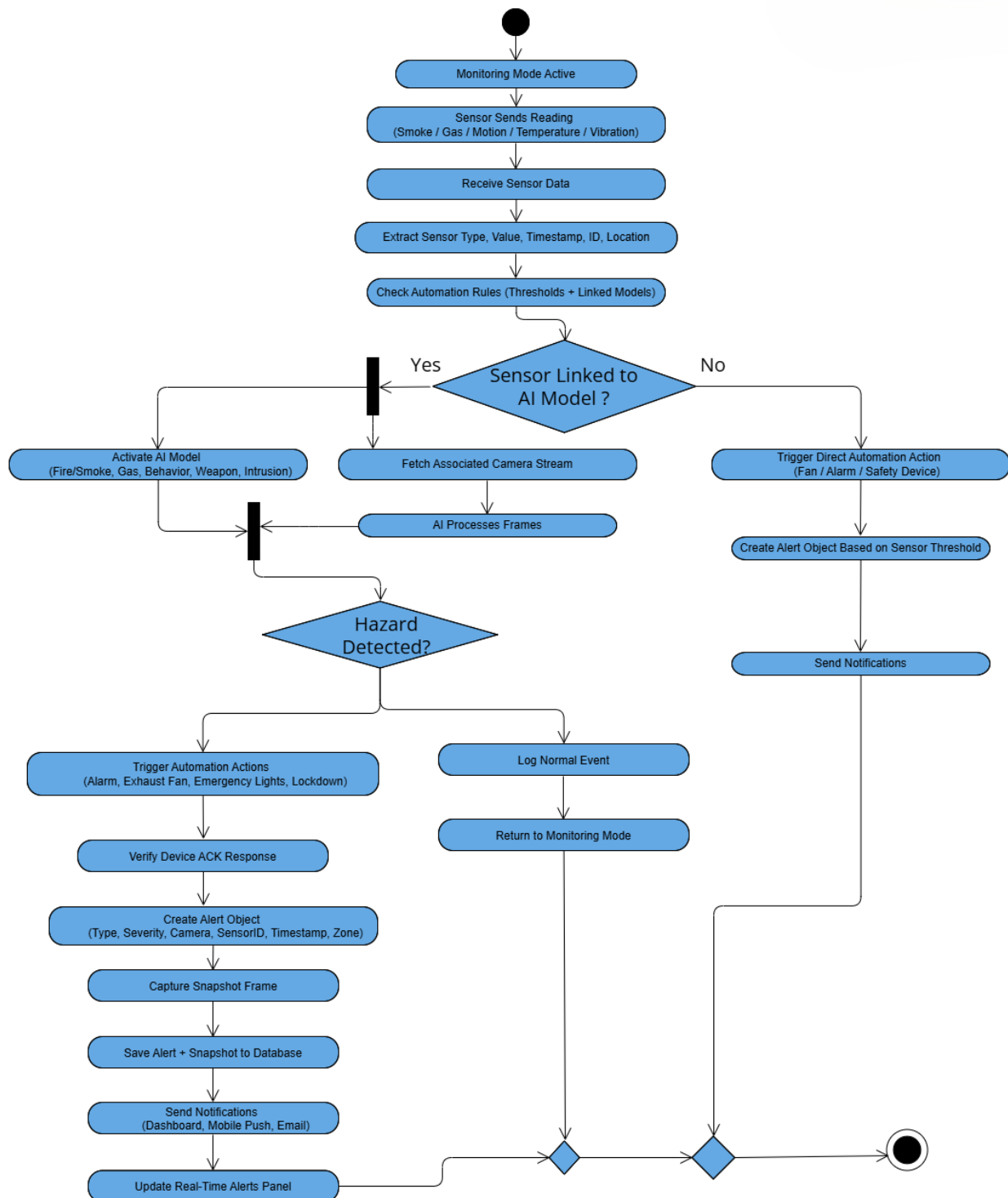
Figure 3.4 : Sensor Trigger & Automation Flow
