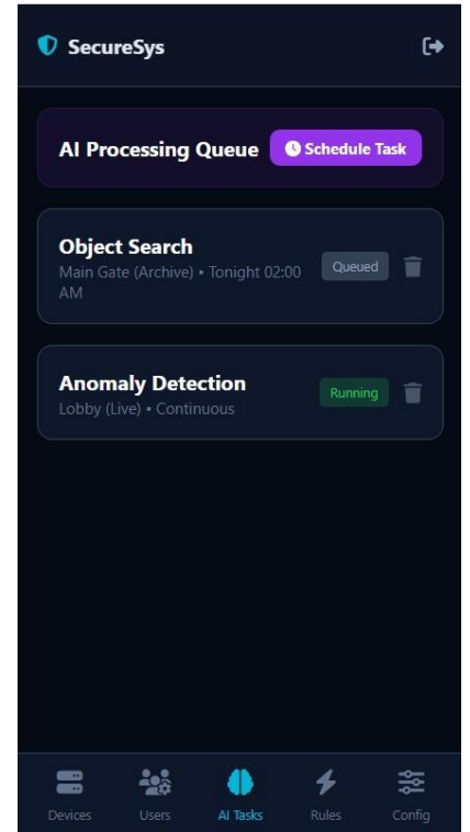
Figure 4.8 : Scheduling Tasks Management UI
