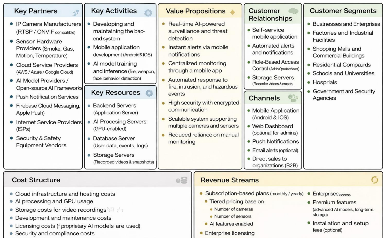
Figure 3.7 : Business Model
