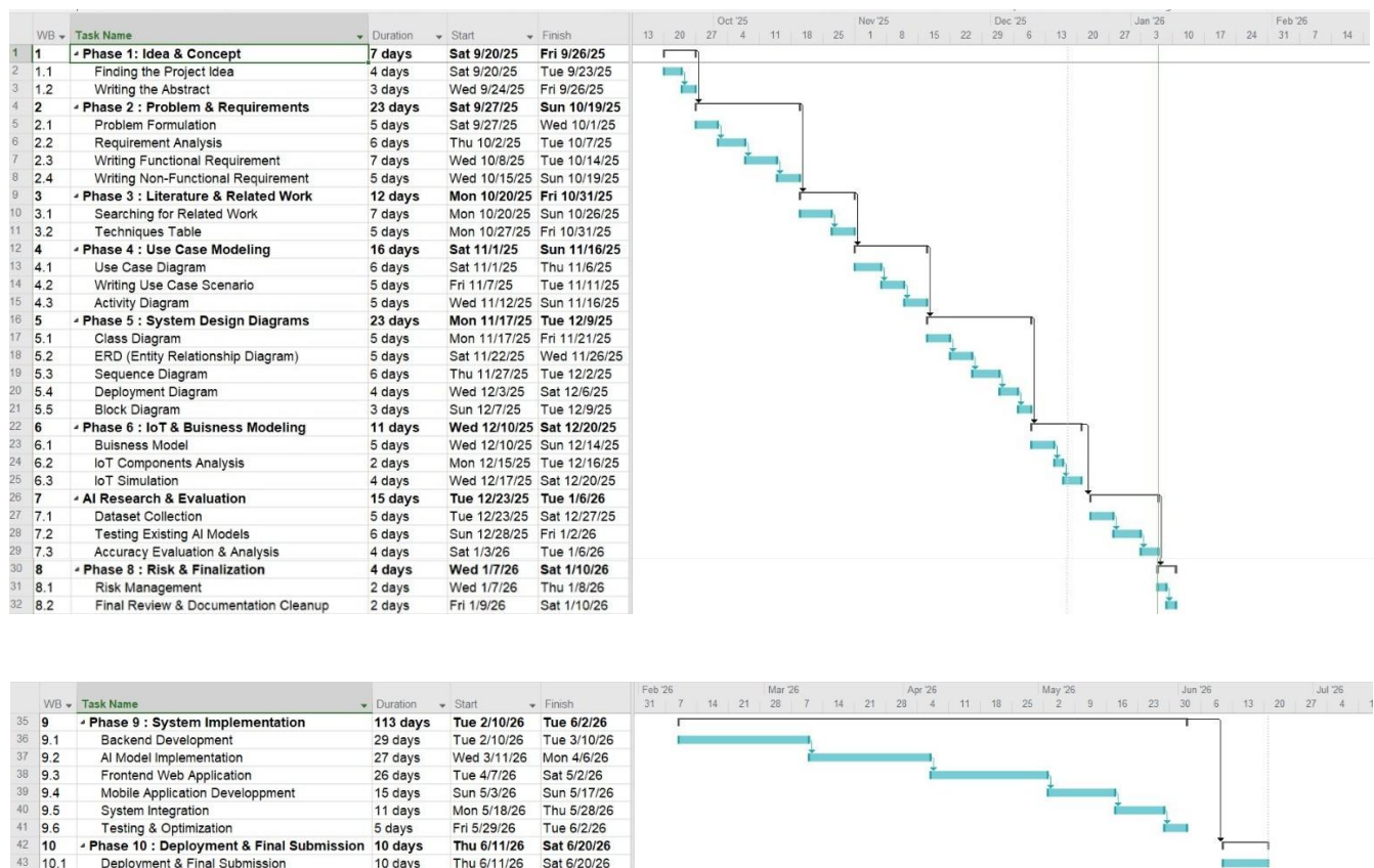
Figure 3.12 : Project Plan
