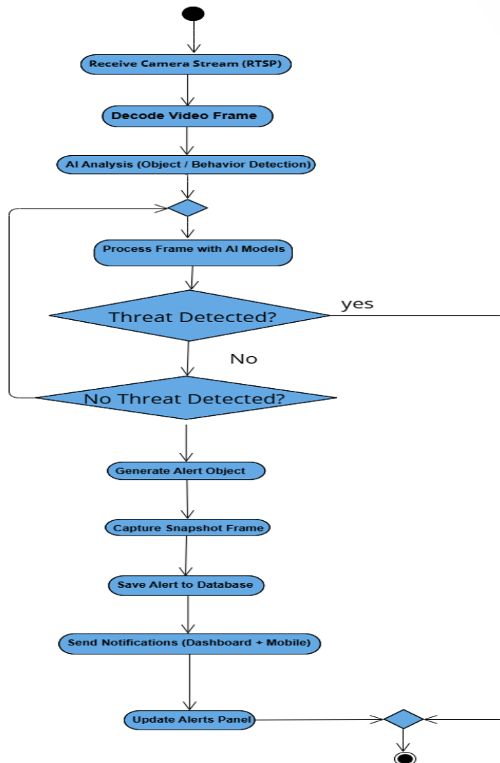
Figure 3.2 : AI Detection & Alert Generation Flow
